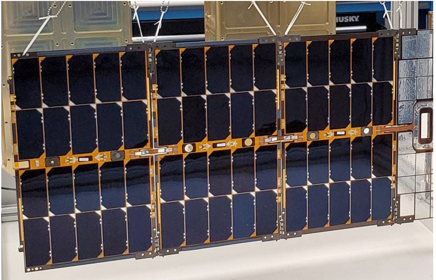
The Pony Express 1 mission is a hosted payload on Tyvak-0129, a next-generation Tyvak 6U spacecraft. Image Courtesy: Tyvak Nano-Satellite Systems, Inc.
