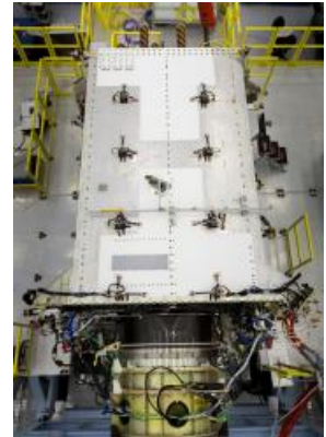
The U.S. Air Force's second GPS III satellite, GPS III SV02, is fully integrated and ready for environmental tests this summer at Lockheed Martin's GPS III Processing Facility.
